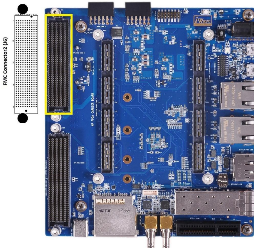
Figure 14: FMC Connector2
